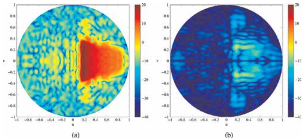
Figure 8. Radiation pattern in the whole visible region radiated by the reflectarray designed for a 5G base station for polarization X. (a) Copolar component of the far field. (b) Crosspolar component of the far field.
