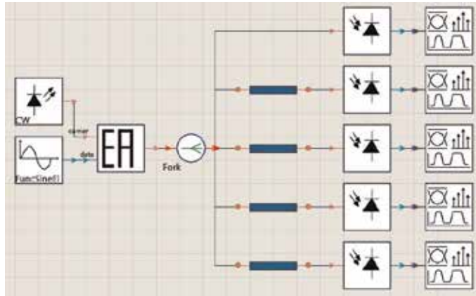
Figure 13. Equivalent delay elements of integrated OBM.
