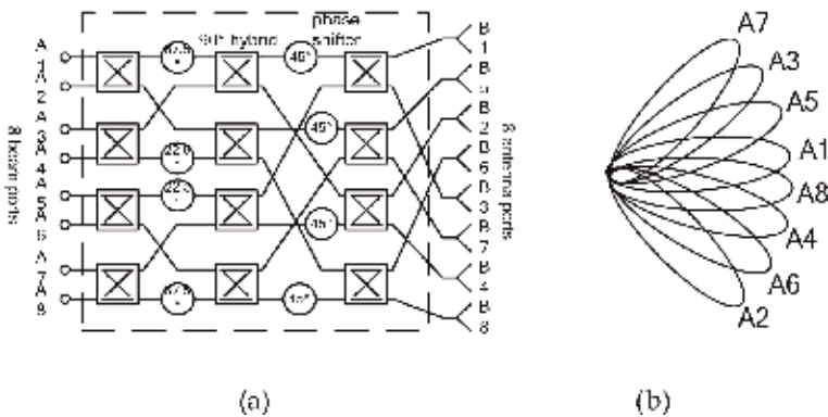
Figure 3. (a) Block diagram of 8×8 traditional Butler matrix and (b) corresponding BFN beam rosette.
