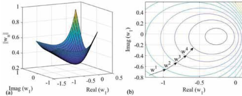
Figure 3. (a) 3D plot of the objective function plotted as a function of real ( w_1 ) and imaginary ( w_1 ). (b) the contour plot of the objective function with illustration of gradient descent method.
