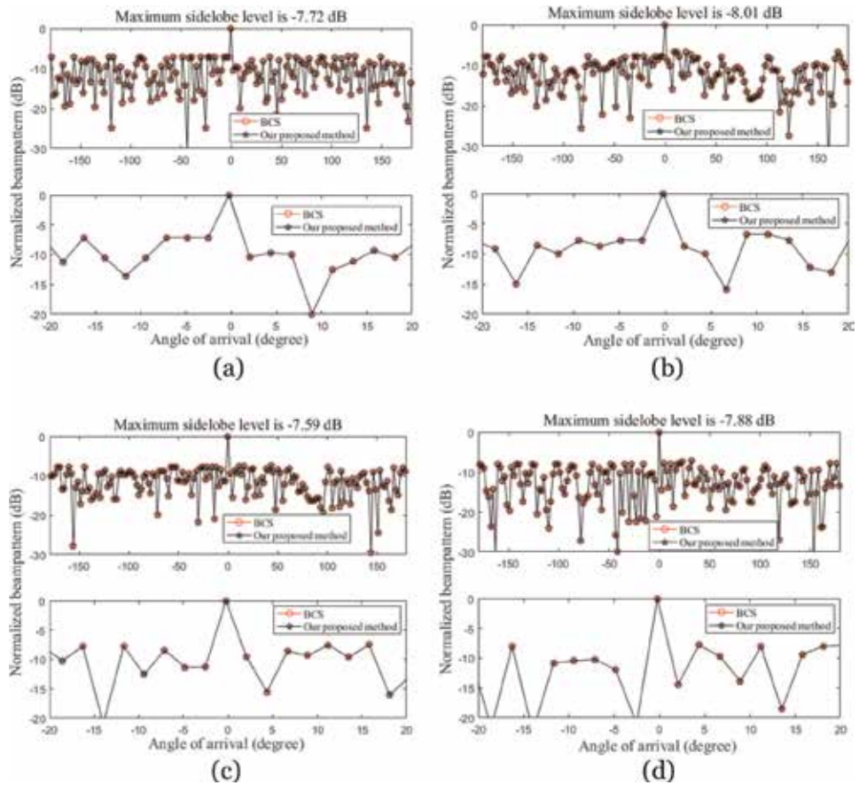
Figure 9. Optimal beam pattern of different element number array by using “BCS inversion algorithm [17]” vs. “our method.” (a) 1 array orientation, (b) 2 array orientations, (c) 3 array orientations, and (d) 4 array orientations.
