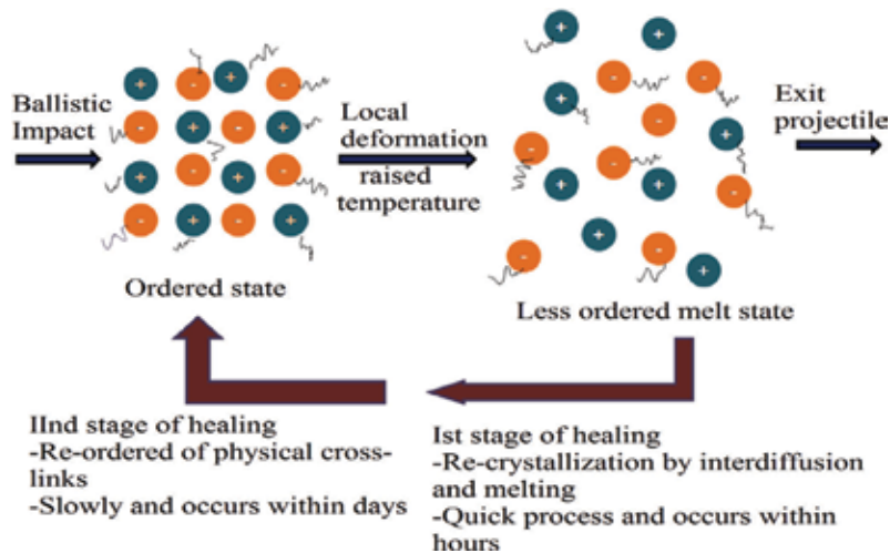
Figure 9. Schematic diagram of ionomeric healing upon ballistic impact based on order-disorder theory of healing presented by Fall [27].
