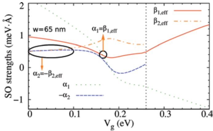
Figure 4. The dependence of intrasubband Rashba \alpha_v and renormalized Dresselhaus \beta_{v,\text{eff}} coefficients on V_g for the 65-nm well. The vertical dashed line marks regions of one- and two-band occupations. The temperature is held fixed at 0.3 K, from Wang et al. [32].
