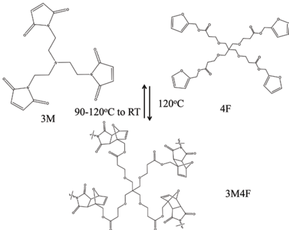
Figure 7. Reversible cross-linked furan-maleimide-based polymer network [18].
