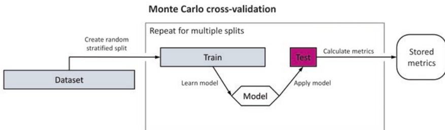
Fig. 8.7 Schematic overview of a Monte Carlo cross-validation. A random stratified split is applied to separate a test set from the training set. A prediction model is trained on the training set and performance metrics on the test set are stored after which the process is repeated
