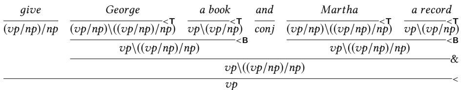
Figure 21.14: Gapping in Categorial Grammar
