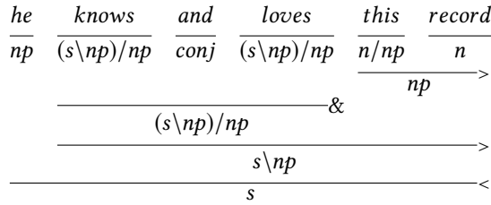
Figure 21.13: Coordination of two transitive verbs in Categorial Grammar
