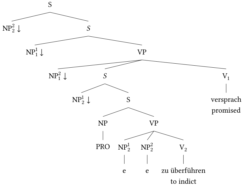
Figure 12.10: Analysis of the order NP_2^2 NP_1^1 NP_1^2 NP_2^1 V_2 V_1 : adjunction to the S node between NP_2^2 and NP_1^1
