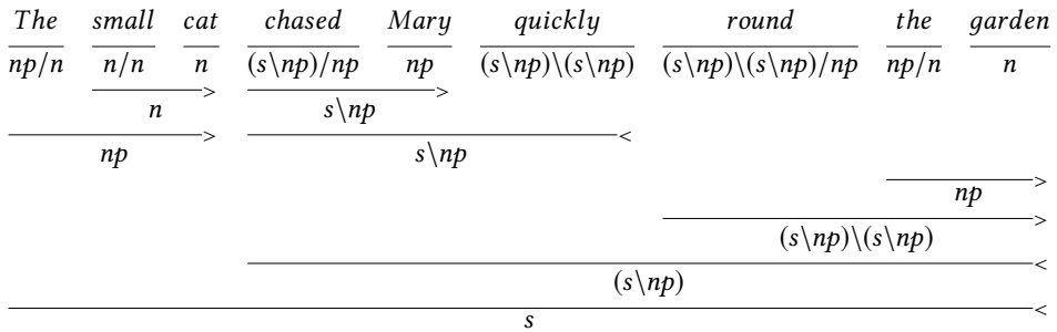
Figure 8.5: Example of an analysis with adjuncts in Categorial Grammar
