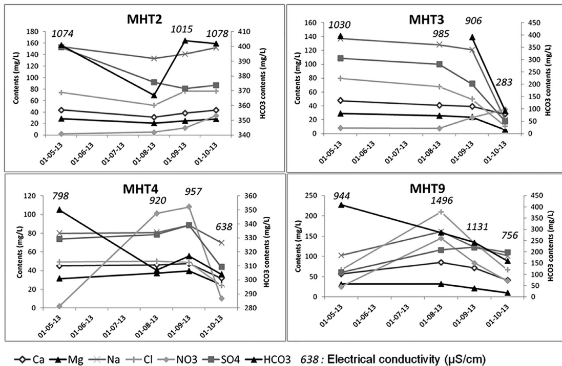
Figure 7.12 Evolution of calcium ( \text{Ca}^{2+} ), magnesium ( \text{Mg}^{2+} ), sodium ( \text{Na}^+ ), chloride ( \text{Cl}^- ), nitrate ( \text{NO}_3^- ), sulphate ( \text{SO}_4^{2-} ) and hydrogen carbonate ( \text{HCO}_3^- ) contents (mg/L) for the campaigns of May (i.e. before monsoon), August and September (i.e. early stages of the monsoon), and October 2013 (i.e. late stage of the monsoon) with the corresponding electrical conductivity.
