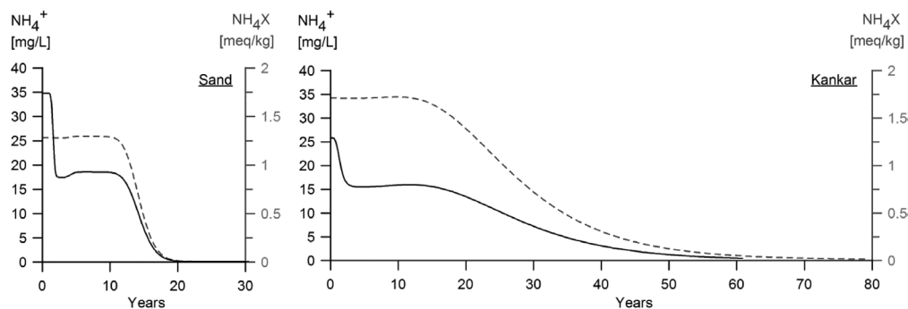
Figure 4.7 Results of the desorption modelling. Solid black line: Ammonium concentration in water in mg/L (shown on the primary y-axis), dashed grey line: Ammonium concentrations on the exchanger in meq/kg sediment (shown on the secondary y-axis). Like in the adsorption-model runs, more ammonium is adsorbed on the kankar material than on the sand. However, the actual amounts adsorbed in the beginning of the desorption-model run are higher than the amounts adsorbed in the adsorption-models (Figure 4.6). The reason for this discrepancy is that the desorption-model was equilibrated with higher concentrations of ammonium (see Table 4.6).
