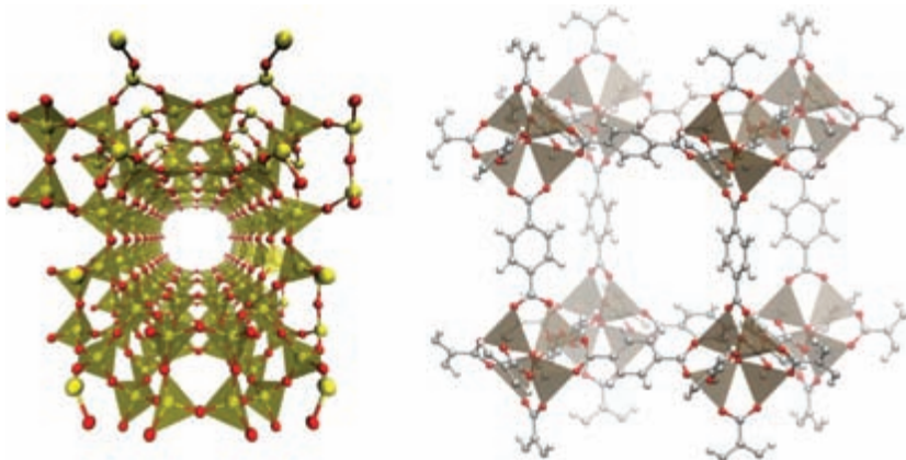
Figure 7. Left: structure of MOR framework. Silicon atoms (shown as yellow spheres) are located in the centres of the tetrahedra (T-sites). Oxygen atoms are shown as red spheres. Right: structure of MOF-5. ZnO nodes represented as tetrahedra, which are interconnected by the terephthalate linkers.
