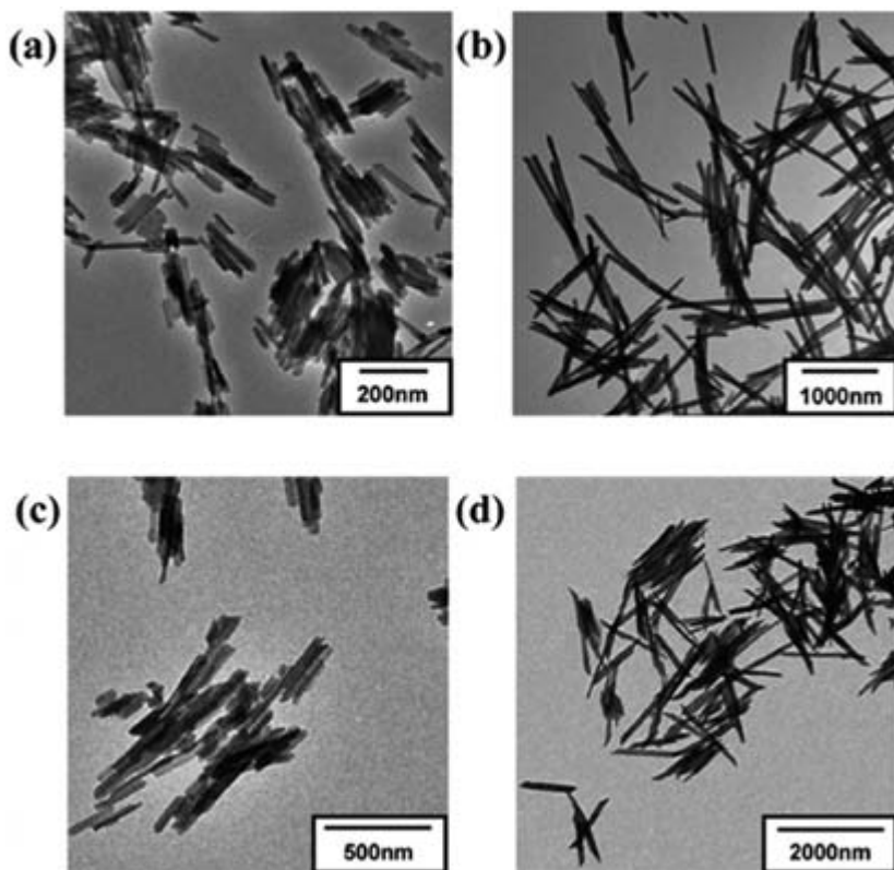
Figure 2. Transmission electron microscopy of 1,4-BDC and Gd^{3+} MOFs with different shapes and sizes. Reprinted with permission from ref. 10. Copyright 2011 American Chemical Society.
