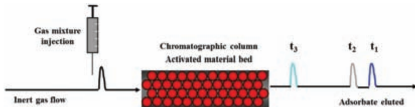
Figure 4. Scheme of the Inverse Gas Chromatography method.
