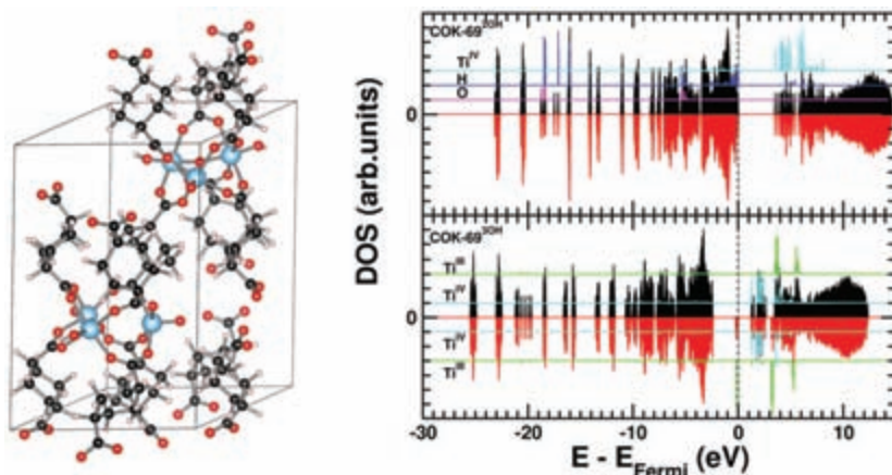
Figure 10. Left: ball-and-stick representation of the primitive unit cell of the COK-69(Ti) MOF. Atomic positions of Ti are indicated in blue. Right: spin polarized DOS of the COK-69(Ti) with different titanium clusters. In the case of COK-69 2OH , each Ti-cluster has two hydroxy groups, leading to three Ti IV atoms, while the Ti-clusters of COK-69 3OH have three hydroxy groups, giving rise to a single Ti III in each cluster. This Ti III gives rise to a gap state and luminescent behaviour.
