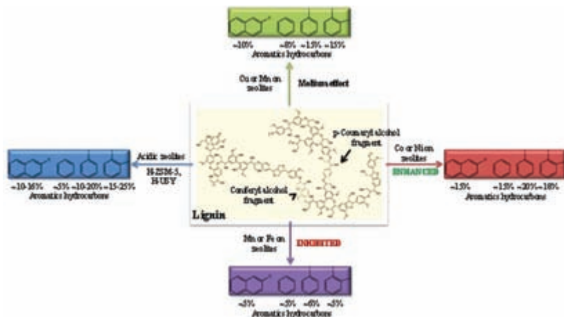
Figure 7. Zeolite transformation of the pyrolysis oil. Copyright © Swiss Chemical Society: CHIMIA, ref. [71]. DOI: https://doi.org/10.2533/chimia.2015.597
