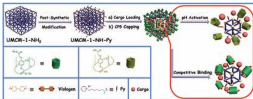
Figure 8. Schematic representation of the stimuli-responsive system based on UMCM-1-NH 2 modified with positively-charged pyridinium (Py) stalks and CP5 on the surface. This system, under pH or competitive binding can regulate the release of cargo molecules. [37] – Published by The Royal Society of Chemistry.
