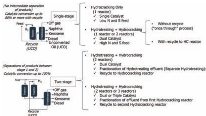
Figure 3. Hydrocracker configurations [22].
