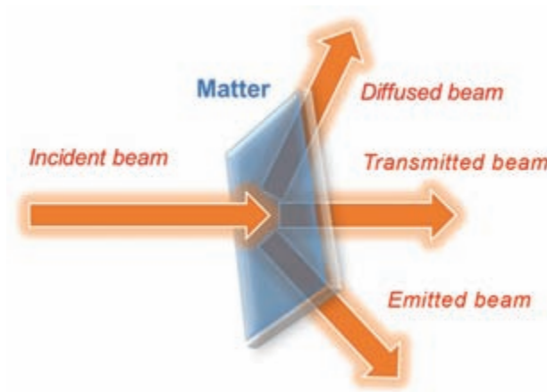
Figure 1. Interaction EMB-matter.
