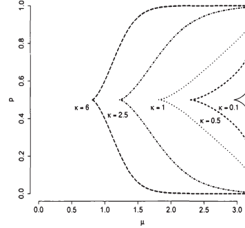
Figure 1.2: Regions of bimodality of the von Mises distribution, where \mu = \mu_2 - \mu_1 and \kappa_1 = \kappa_2 = \kappa . On the right side of the curves are those parameter constellations of p and \mu for which for fixed \kappa the resulting mixture is bimodal.
