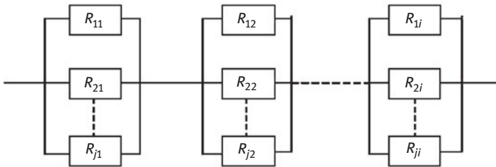
Figure 10.14: Series—parallel system.
