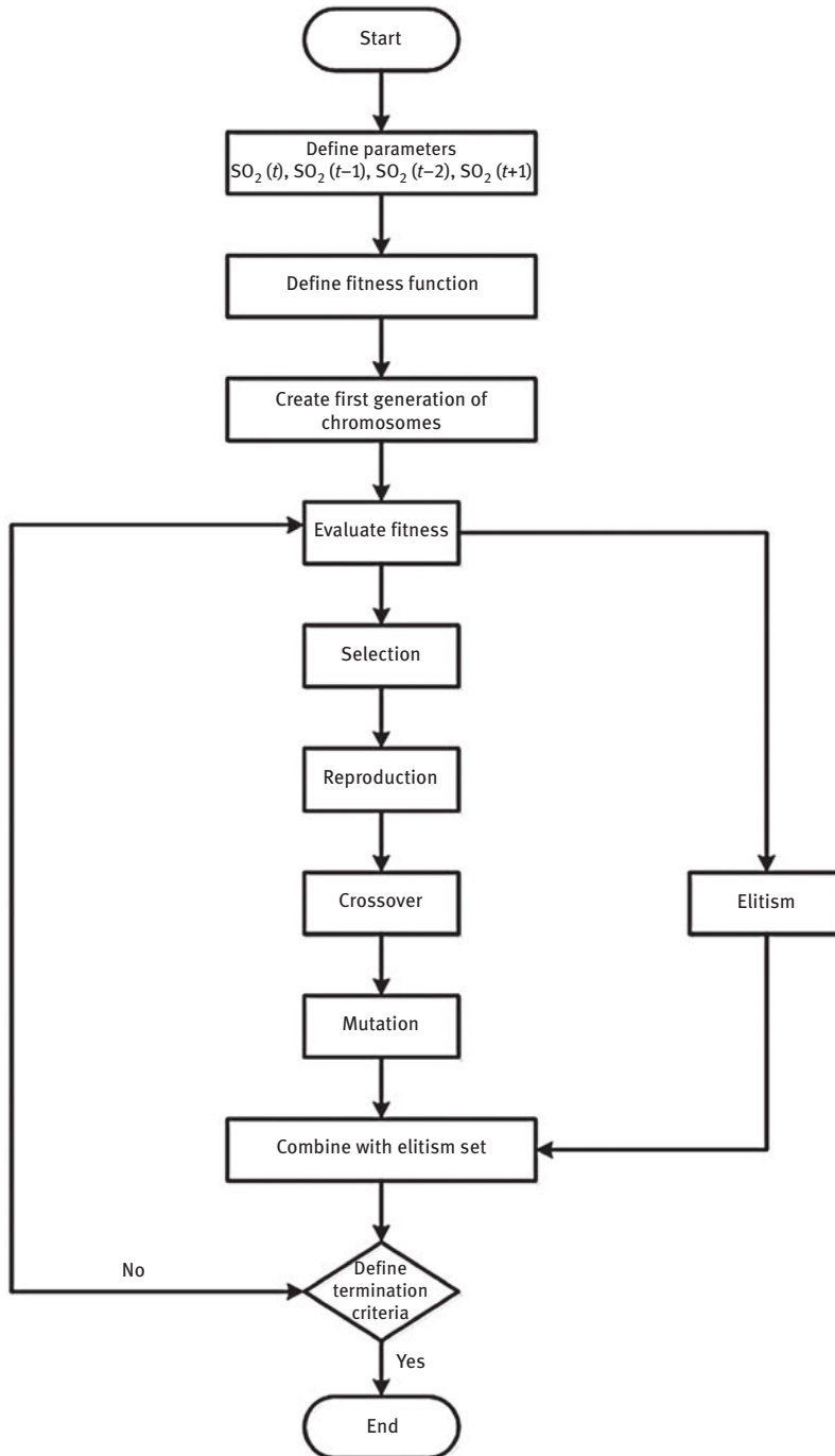
Figure 6.2: Typical GP Flowchart. Source: Yadav & Sharma, 2019.
