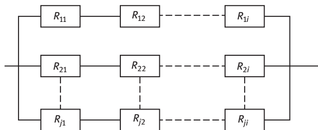
Figure 10.9: Parallel-series system.
