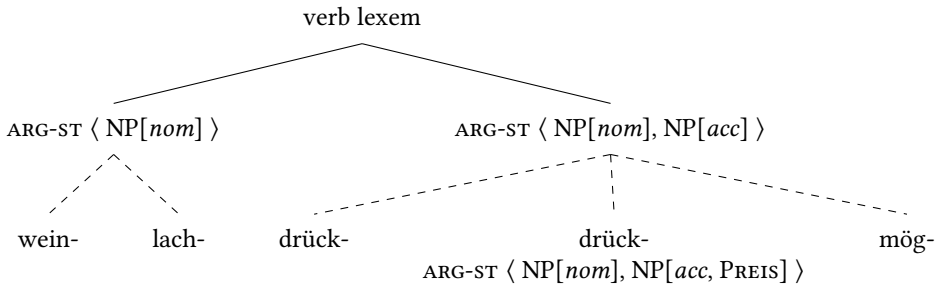
Figure 21.9: Lexical alternative to inheritance hierarchy in Figure 21.8
