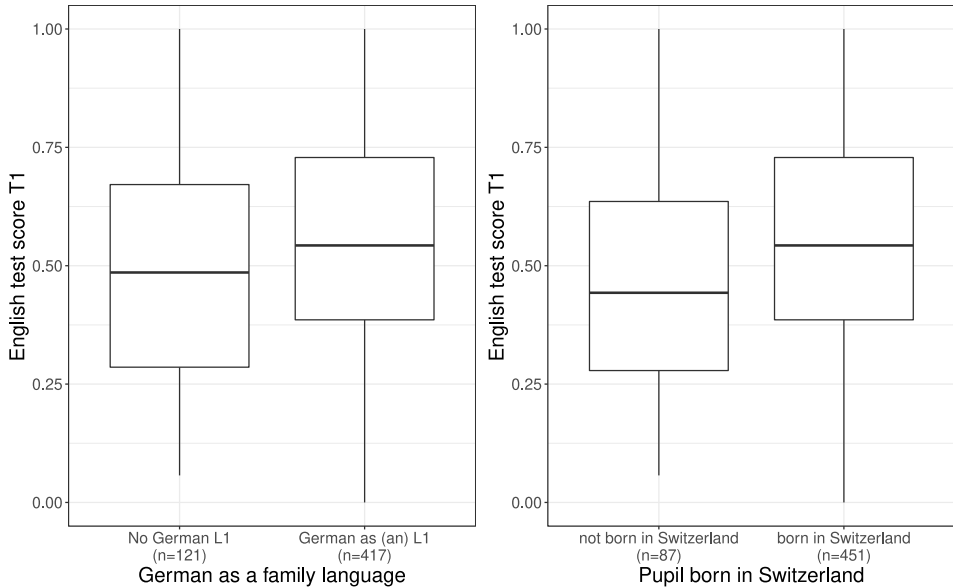
Figure 2: English scores at T1 and either German as a home language (left) or country of birth of the children (right).
