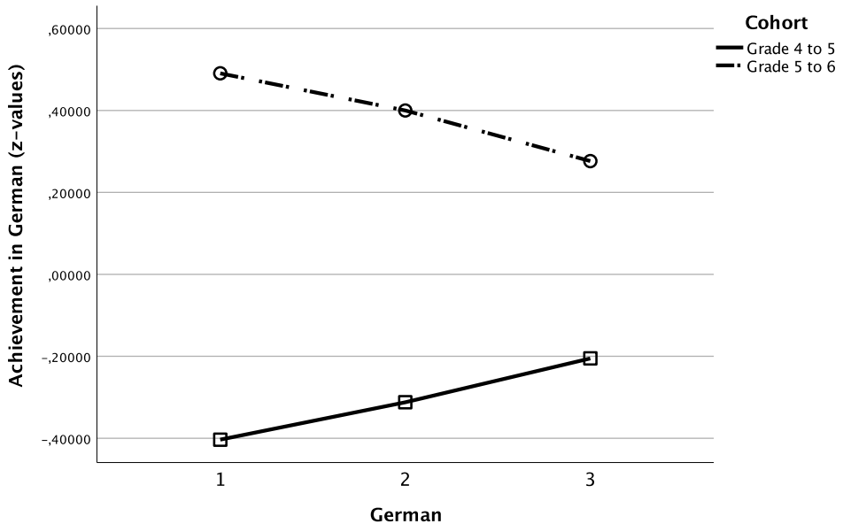
Figure 2: The development of test results in German (standardized measures of the ELFE-subtest on sentence reading) T1 to T3 for the two age groups (grades 4 to 5, grades 5 to 6); Repeated Measures ANOVA: within subjects (measurements T1-T3)*between subject (age groups) effects significant (Greenhouse-Geisser, F = 22.53, df = 1.94, p < 0.001 ); covariates: fluid intelligence CFT 20 ( F = 64.86, p < 0.001 ); SES ( F = 52.76, df = 1, p < 0.001 )
