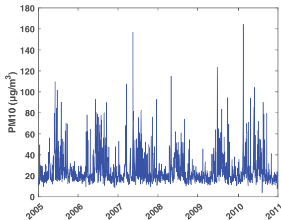
Figure 1. Illustration of PM10 daily average concentrations between 2005 and 2010, highlighting intermittent burst events with huge fluctuations.
