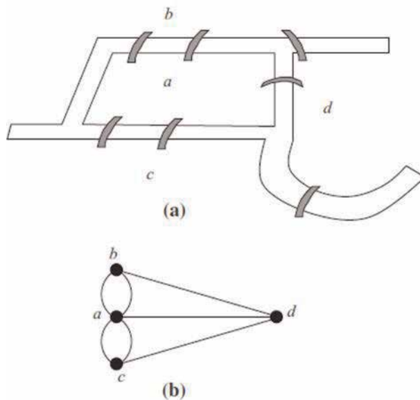
Figure 1. Königsberg seven-bridge problem.
