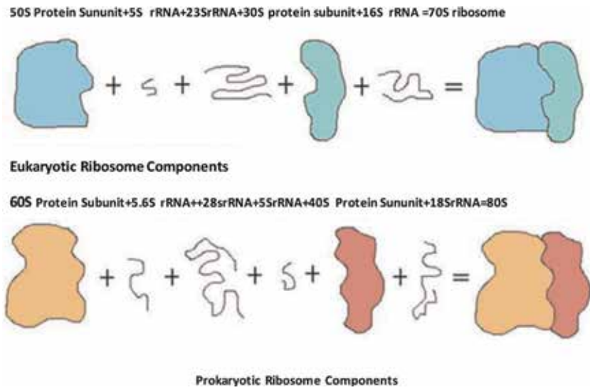
Figure 6. Prokaryotic ribosome components.
