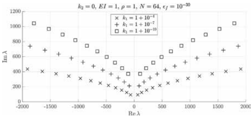
Figure 6. Eigenvalues with |\text{Re}\lambda| > 10 as k_1 \rightarrow 1^+ .
