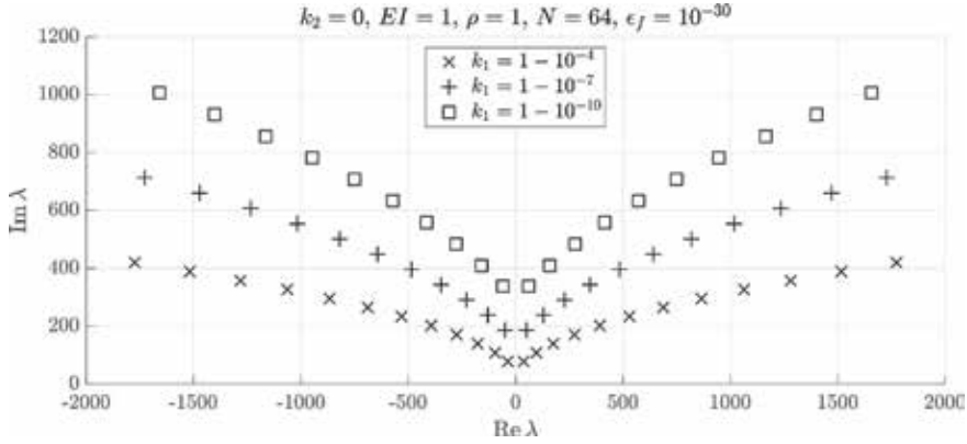
Figure 7. Eigenvalues with |\operatorname{Re} \lambda| > 10 as k_1 \rightarrow 1^- .
