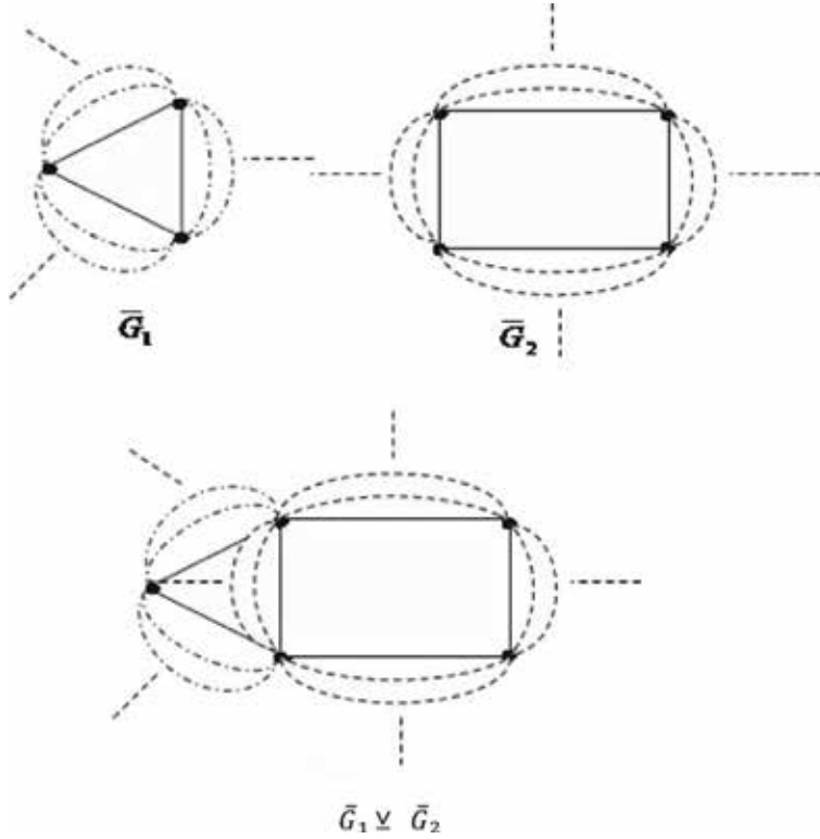
Figure 3. Chaotic connected edge.
