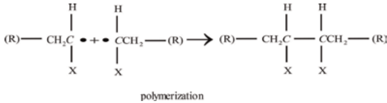
Figure 4. Polymerization.
