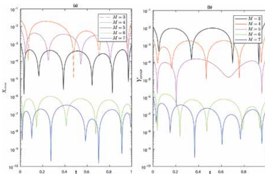
Figure 6. Absolute error in approximate solutions at different scale level M = 3:7 for Example 4.3.
